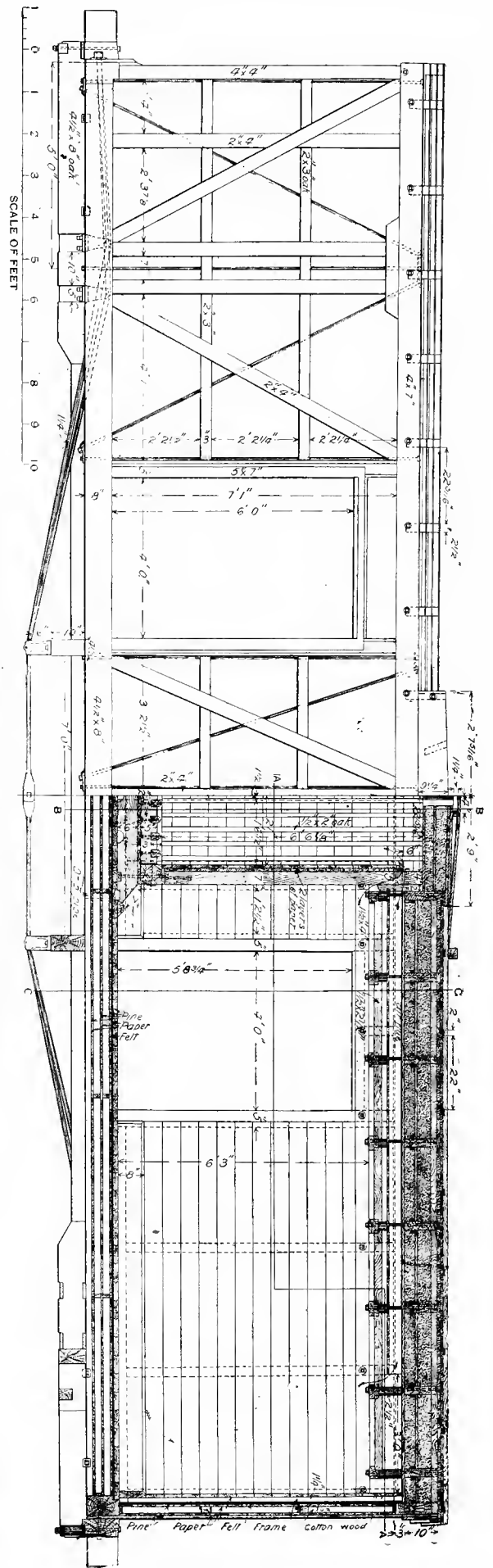
Fig. 274. Half Side Elevation of Fronting and Half Longitudinal Section.
